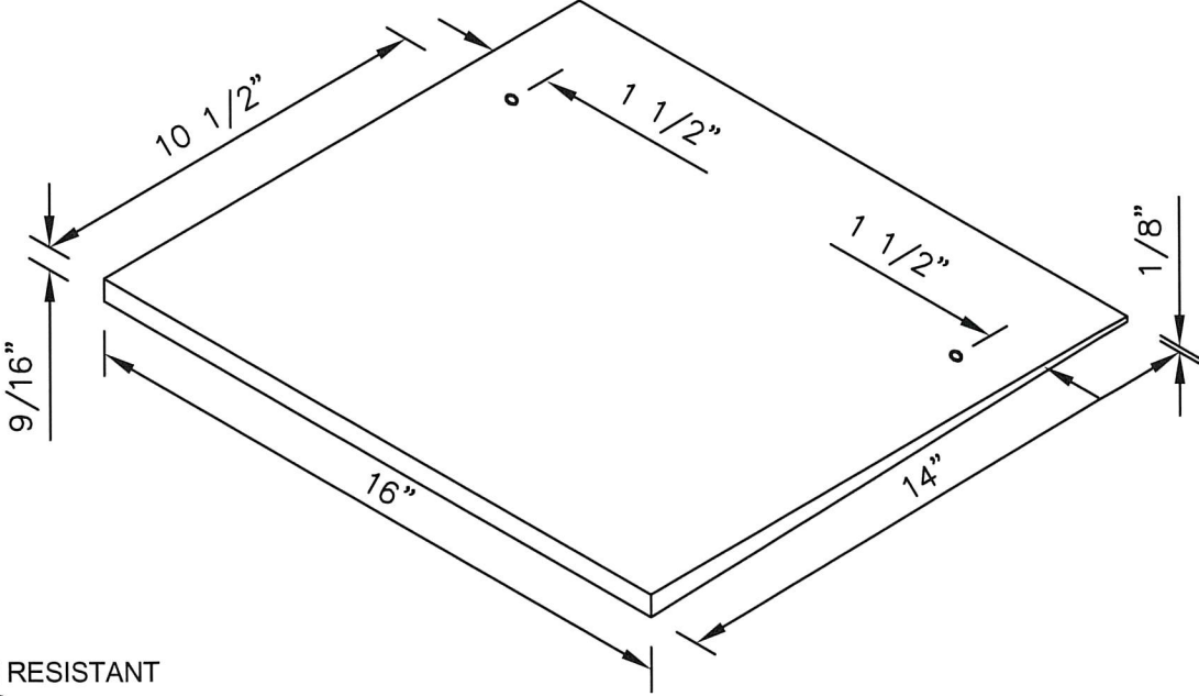
EAVE STARTER
